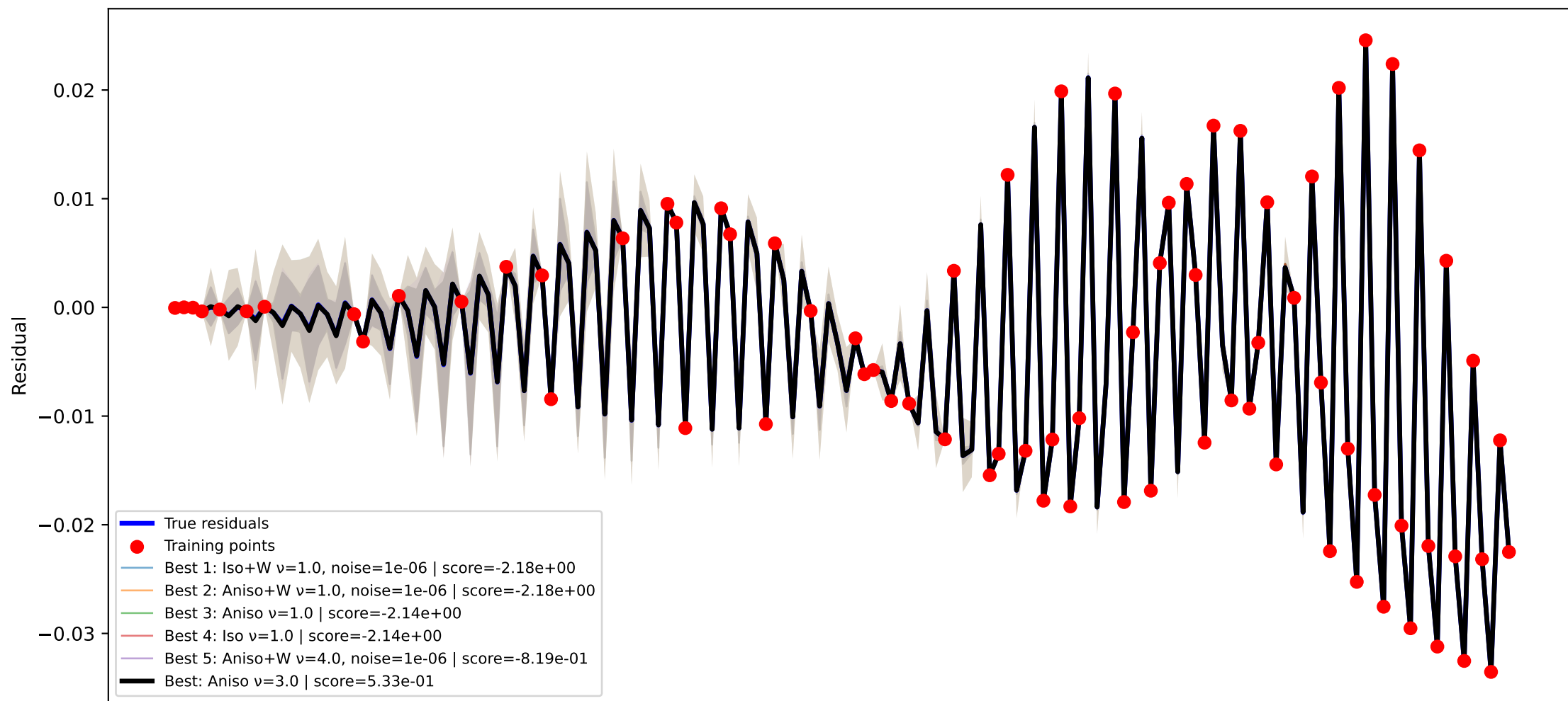
GPR kernel comparison node=17 RMSE=2.664e-05, train RMSE=3.164e-11
